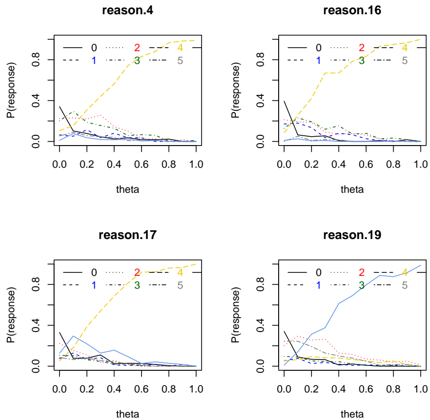
Figure 15: The pattern of responses to multiple choice ability items can show that some items have poor distractors. This may be done by using the irt.responses function. A good distractor is one that is negatively related to ability.
